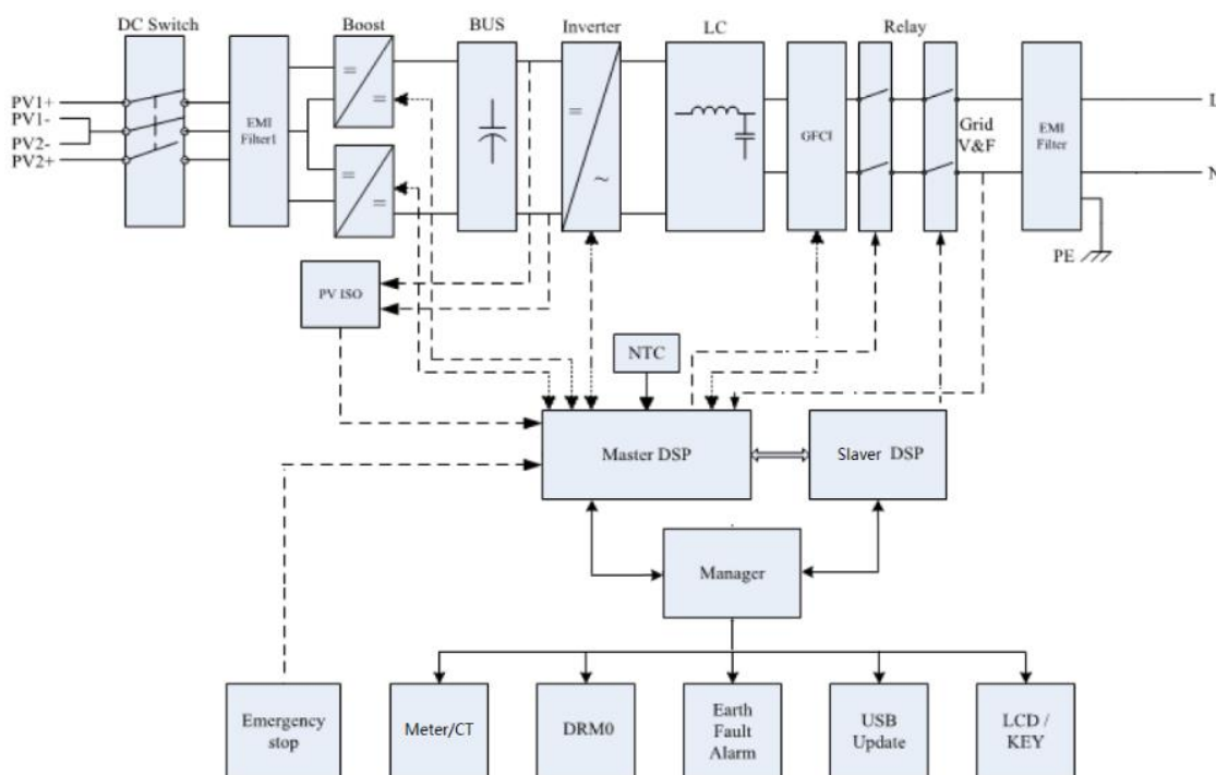
Block diagram:
