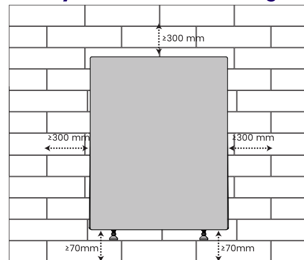
Wall mounting
