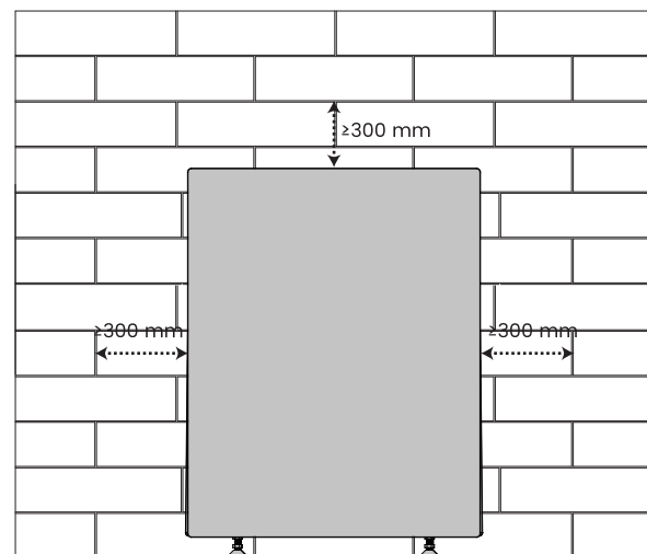
Standing mounting
