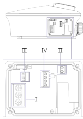
Single phase(7.3kW)
