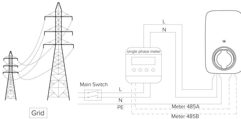
Single phase(7.3kW)
