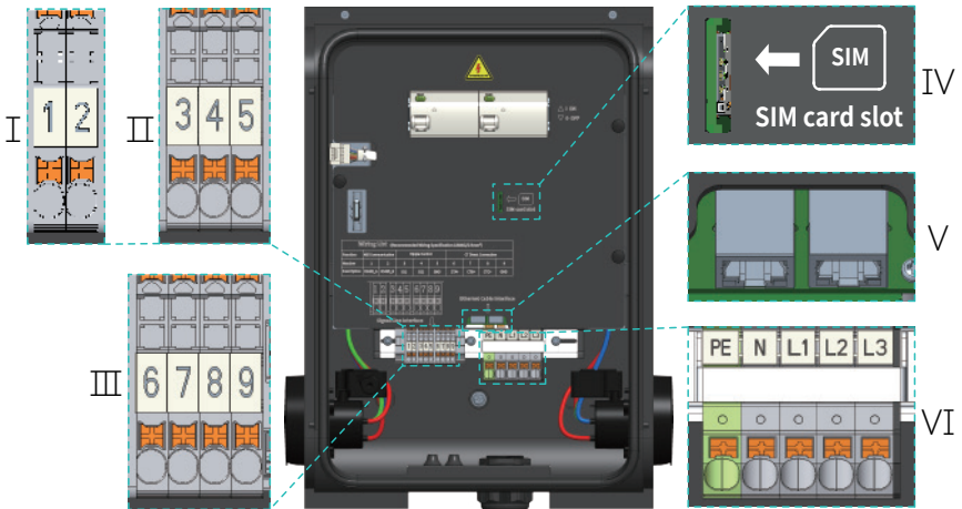
Three phase(11kW*2 & 22kW*2)
