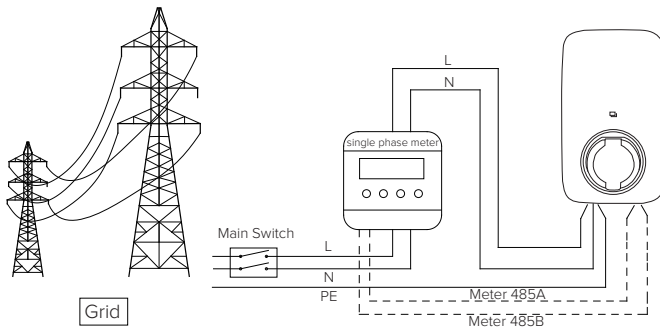
Single phase(7.3kW)
